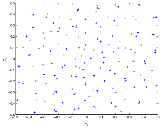
(b) L = 6
