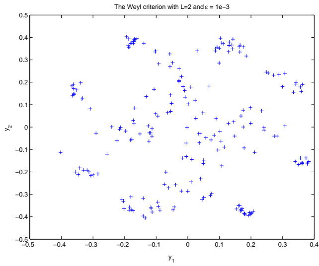
(a) L = 2
