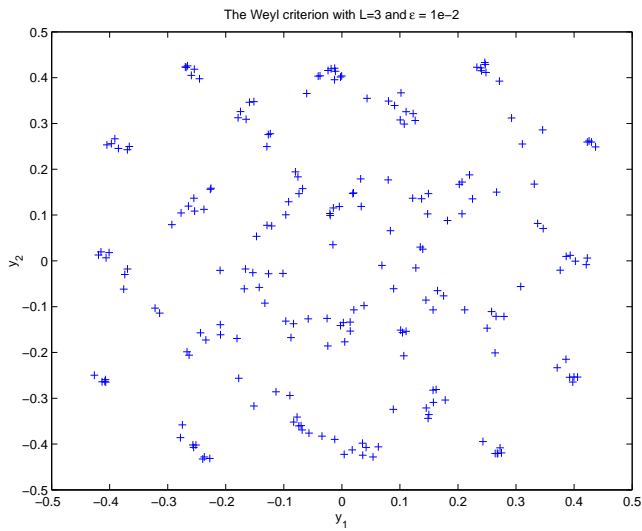
(a) \epsilon = 10^{-2}
